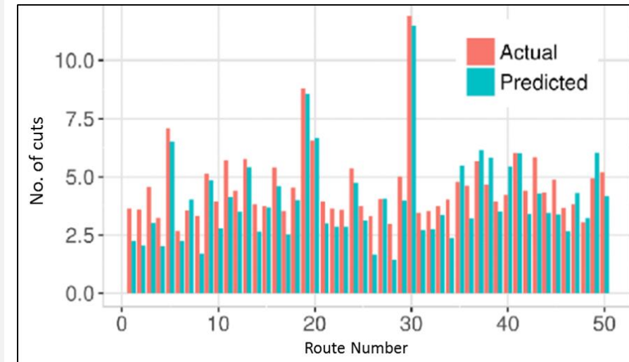
2. Prediction of fiber cuts
